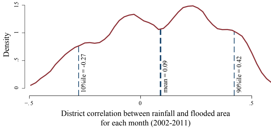
Figure 1: Distribution of correlation coefficients, \rho(flood_i, rain_i) for all districts, i , in Bangladesh for each month in our dataset.
