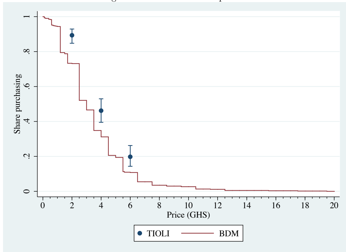
Figure 3: BDM-TIOLI Comparison
