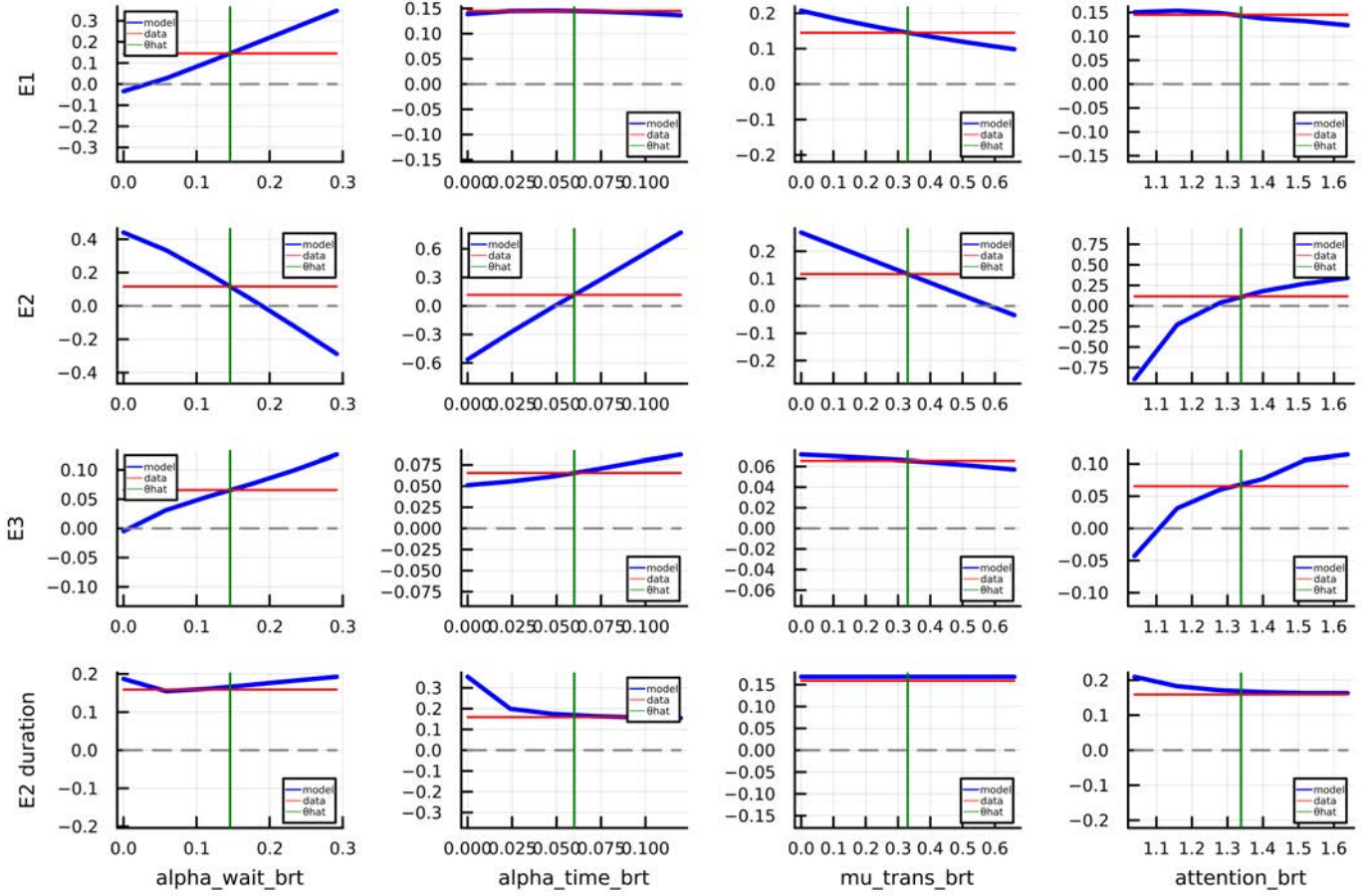
Figure A.9: Moment Dependence on Parameters (Jacobian)
