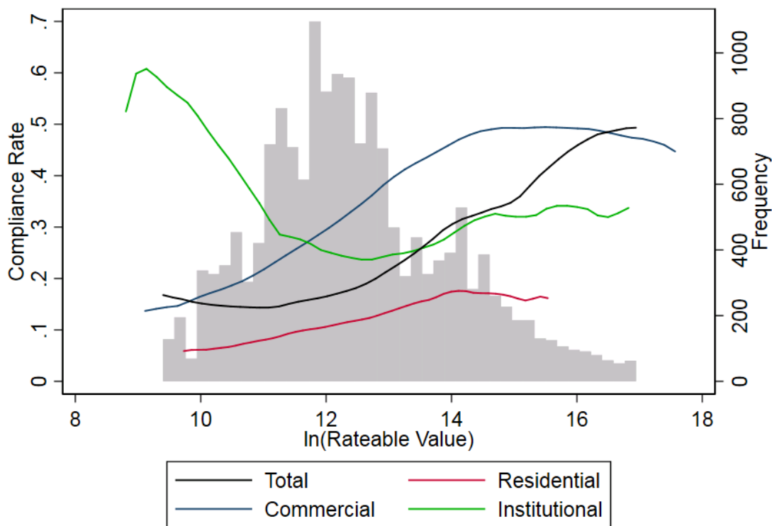
Figure 5: Tax compliance in Central division vs rateable value and property type
