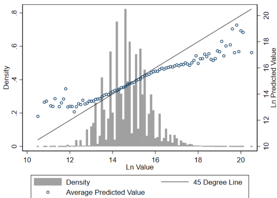
Figure 4: Residential model 2a, calibrated with a 5% sample by division
