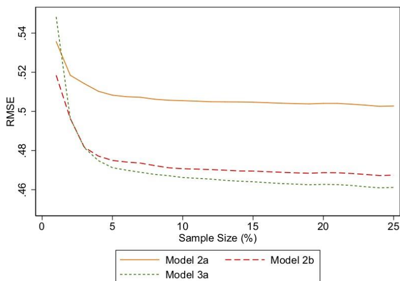
Figure 3: Out of calibration sample average error by sample size, residential properties
