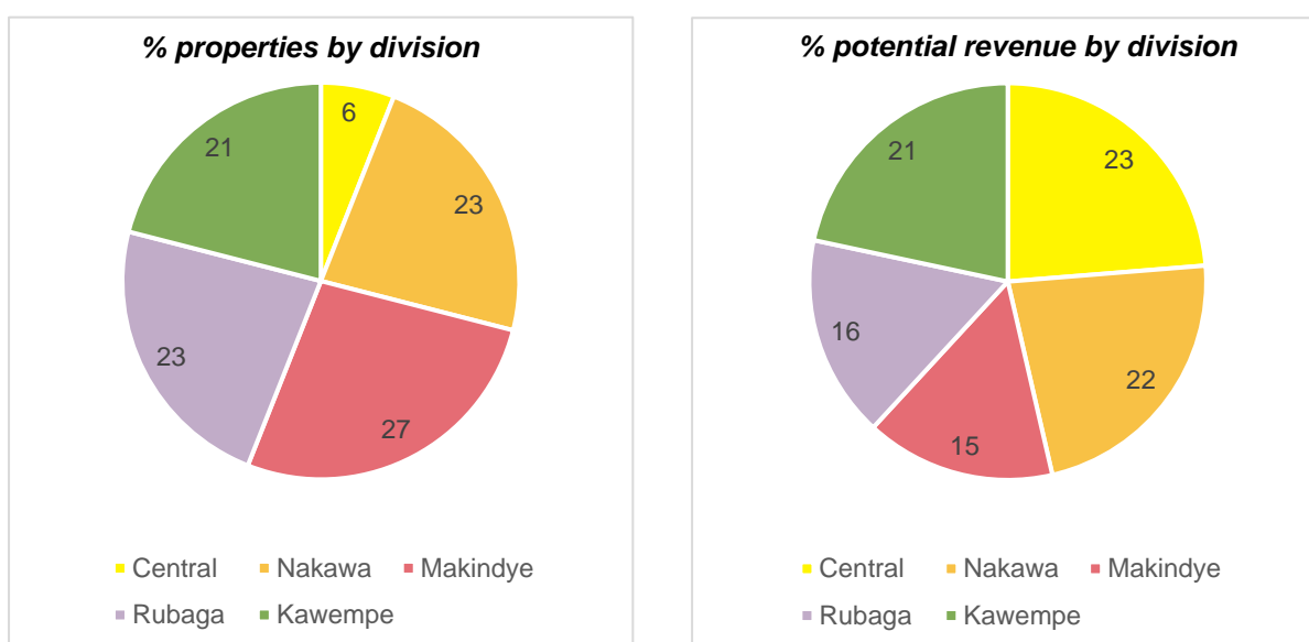
Figures 1: Percentage of properties by division and potential revenue by division
